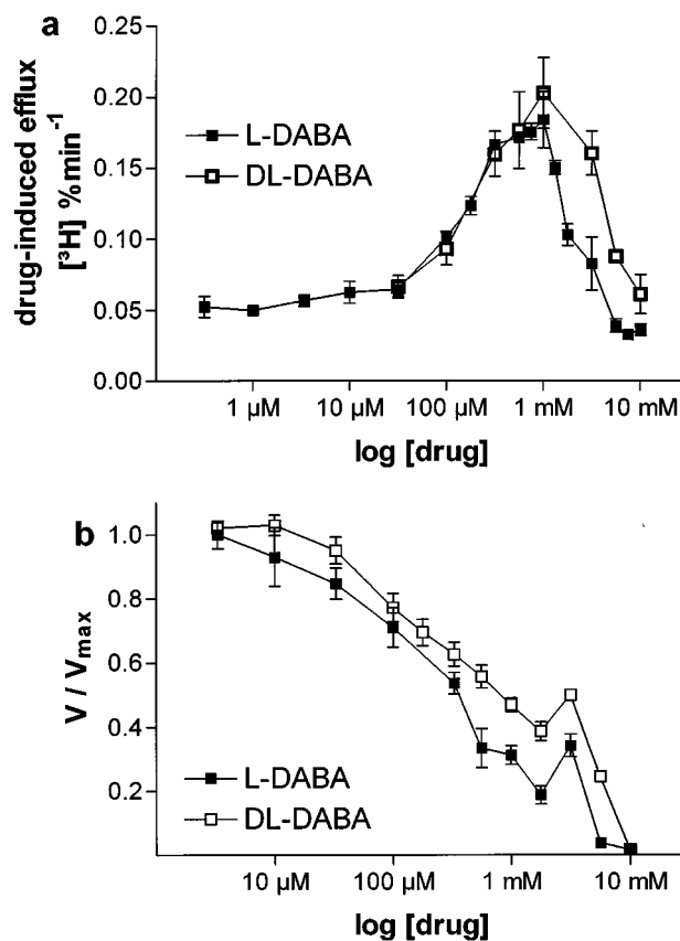
Figure 3 Effect of L- and DL-DABA on uptake and efflux of [^3\text{H}]\text{-GABA} in HEK-293 cells stably expressing the rGAT-1. (a) Concentration-response curve of L- and DL-DABA for their effects on [^3\text{H}]\text{-GABA} efflux. Experimental details see legend to Figure 2. Symbols represent means \pm s.e. mean of eight observations (four experiments each performed in duplicate). (b) Concentration-inhibition curves of L- and DL-DABA for their effects on [^3\text{H}]\text{-GABA} uptake. Experimental details see legend to Figure 2. Symbols represent means \pm s.e. mean of 12 observations (four experiments each performed in triplicate).
