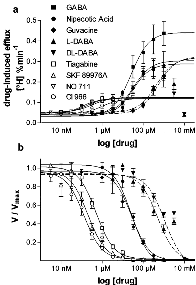
Figure 2 Effect of substrates and re-uptake-inhibitors on uptake and efflux of [^3\text{H}]\text{-GABA} in HEK-293 cells stably expressing the rGAT-1. (a) Concentration-response curves of substrates and re-uptake-inhibitors of GAT-1 for their effects on [^3\text{H}]\text{-GABA} efflux. For experimental details see Figure 1. Drug-induced efflux ( \% \text{ min}^{-1} ) was calculated as the mean efflux of fractions 6–8 divided by the length of the fraction ( = 2 \text{ min} ). Symbols represent means \pm s.e. mean of six observations (three experiments each performed in duplicate). The data were fitted by nonlinear regression. \text{EC}_{50} values are given in Table 1. The fits for L-DABA and DL-DABA were done excluding all data points > 1 \text{ mM} (see also Figure 3a). (b) Concentration-inhibition curves of substrates and re-uptake-inhibitors of GAT-1 for their effects on [^3\text{H}]\text{-GABA} uptake. Cells were incubated in 48-well plates ( 5 \times 10^5 cells/well) with 5 \mu\text{M} [^3\text{H}]\text{-GABA} for 3 min at room temperature as described in Methods. Test drugs were added 3 min before [^3\text{H}]\text{-GABA} using at least six different concentrations. Non-specific uptake was measured in the presence of 10 \mu\text{M} tiagabine. Symbols represent means \pm s.e. mean of nine observations (three experiments each performed in triplicate). The data were fitted by non-linear regression. \text{IC}_{50} values are given in Table 1. The fits for L-DABA and DL-DABA was done excluding all data points > 1 \text{ mM} (see also Figure 3b).
